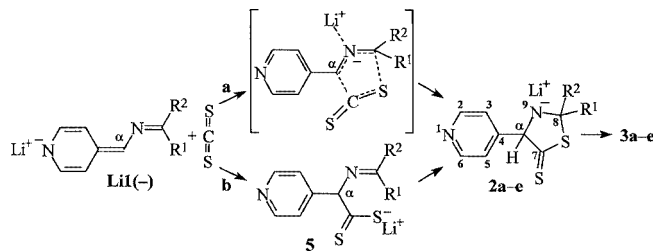
Scheme 3. Only 2e was isolated: Yield 46%. The numbering of 2 does not follow the IUPAC rules, but should facilitate the NMR descriptions.
