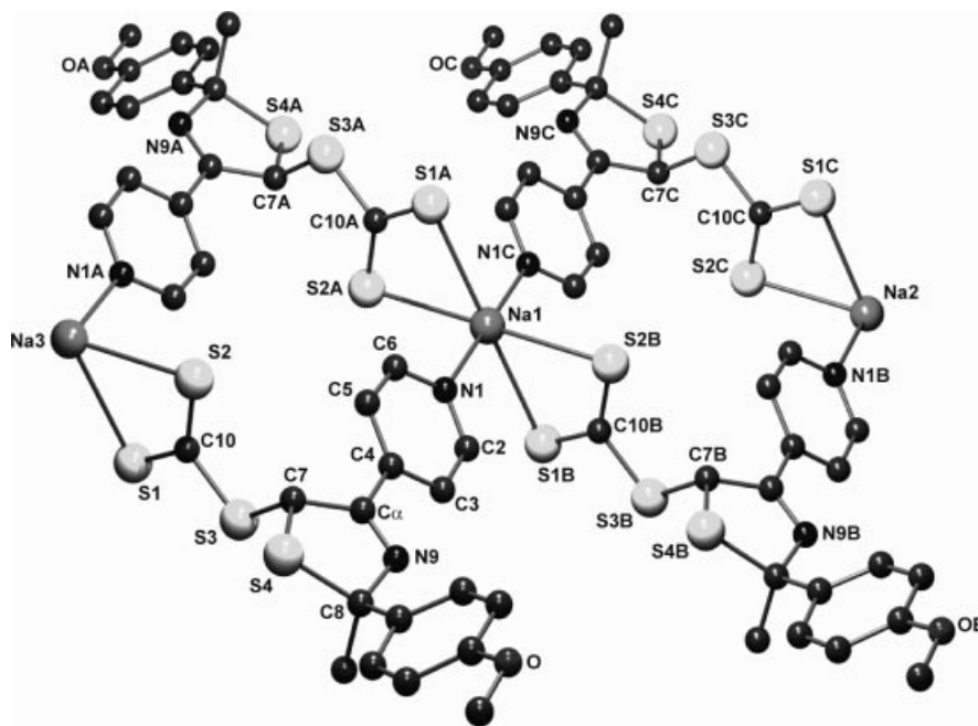
Figure 4. Structure motif of the complex anion \{[\text{Na}_3(\text{trithiocarbonate})_4]^{-}\}_{\infty} of 9 .
