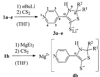
Scheme 2. The numbering of 3 does not follow the IUPAC rules, but should facilitate the NMR descriptions; in the case of 4b \text{MgEt}_2 was used for deprotonation of 1b .
