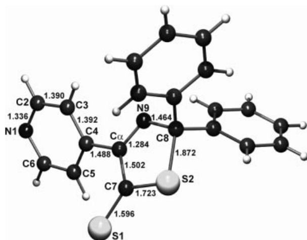
Figure 3. Molecular structure of 7d with selected bond lengths [Å] and angles [°]: C \alpha –N9 1.284, C \alpha –C7 1.502, C7–S1 1.596, C7–S2 1.723, C8–S2 1.872, C8–N9 1.464, C \alpha –C4 1.488; S1–C2–S2 124.6, N9–C \alpha –C7 117.6, N9–C8–S2 106.6, C7–S2–C8 92.5.
