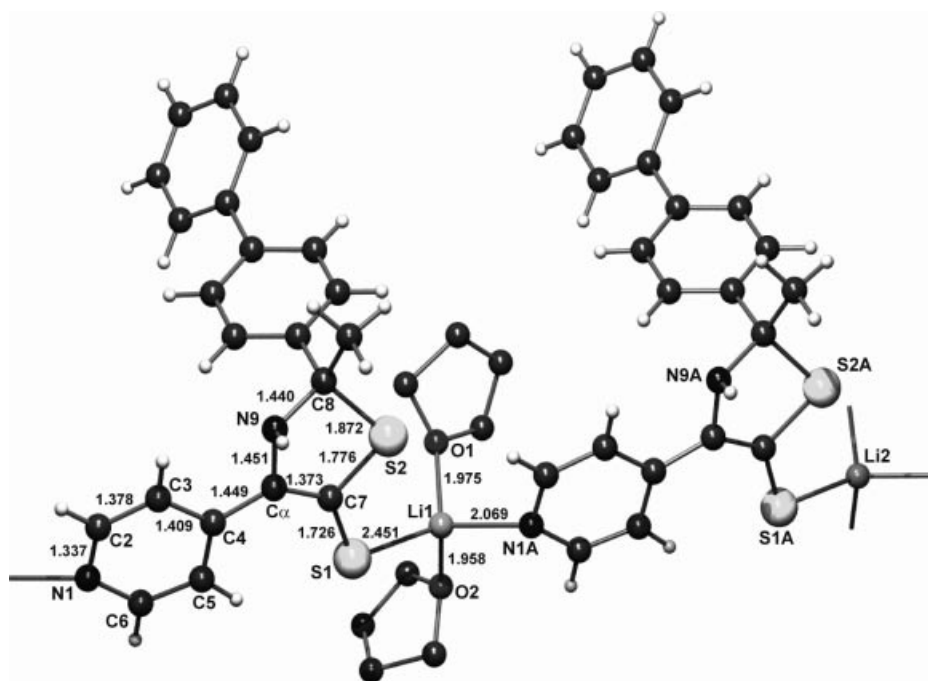
Figure 1. Molecular structure of [\mathbf{3a}(\text{THF})_2]_{\infty} with selected bond lengths [Å] (hydrogen atoms of the solvent molecules are omitted for clarity).
