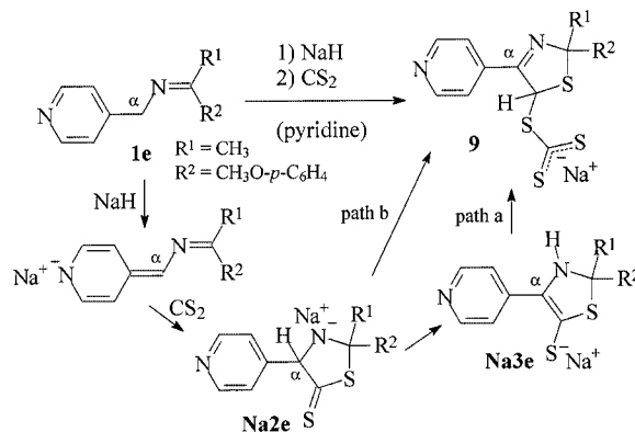
Scheme 6. Two possible reaction pathways a and b for the formation of compound 9 .
