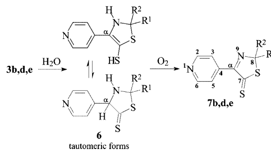
Scheme 4. The numbering of 2 does not follow the IUPAC rules, but should facilitate the NMR descriptions in the Experimental Section.
