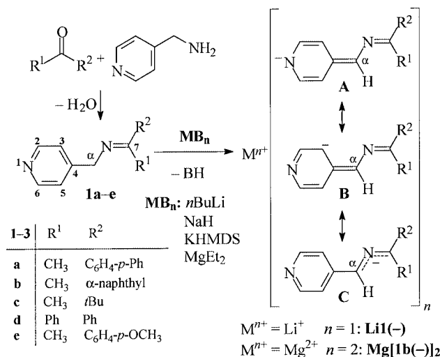
Scheme 1. The ambident anions 1 ( − ) are obtained by deprotonation of the azomethines 1 [derived from different ketones and 4-(aminomethyl)pyridine].
