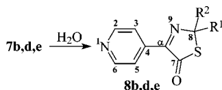
Scheme 5. Hydrolyses of 7b,d,e to the thiazole-5(2 H )-ones 8b,d,e .
