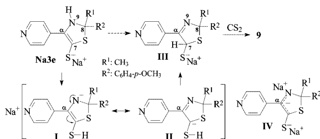
Scheme 7. Possible reaction intermediates in the formation of 9 according to pathway a.
