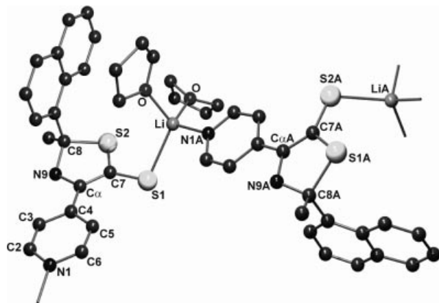
Figure 2. Structure motif of [3b(THF)] 2 (hydrogen atoms are omitted).
